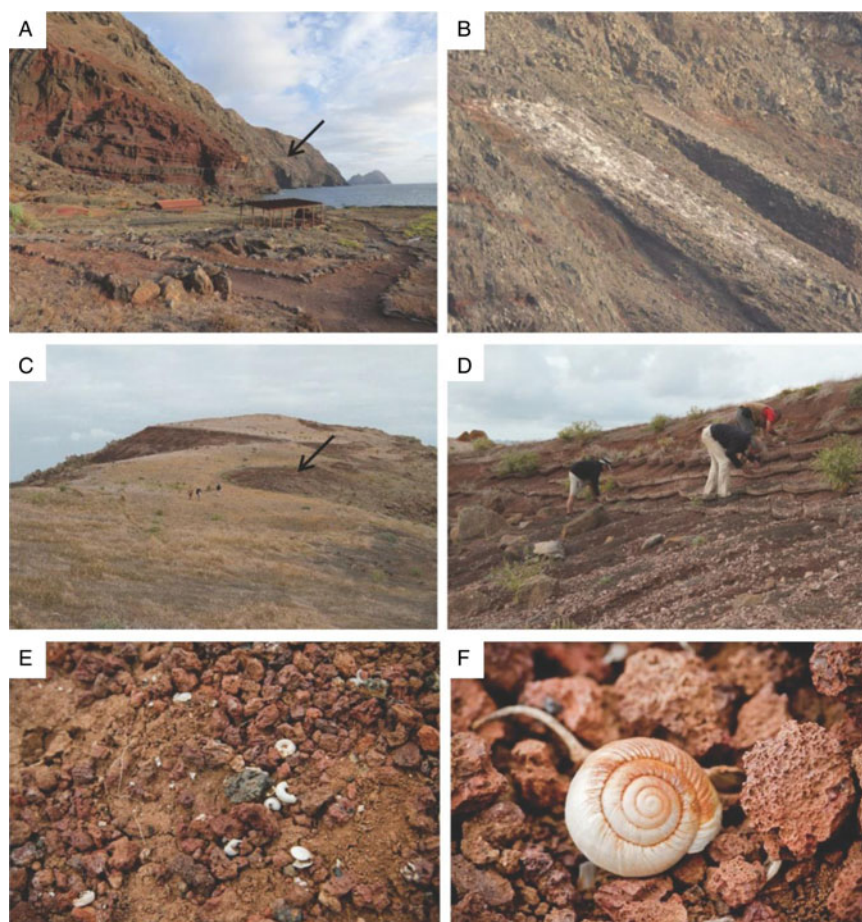
Figure 2. (color online) Field photographs of Quaternary colluvial deposits from the Desertas Islands of the Madeira Archipelago, Portugal. (A) General view of the abrupt volcanic landscape of Deserta Grande Island. Black arrow denotes colluvial sediments from site DG4. (B) Close-up view of the DG4 site in Deserta Grande Island. Shell samples were retrieved from unconsolidated brown-reddish silt-clay sediments on the side base of the slope. (C) Escarpments formed into the flat-topped hill from Bugio Island. Black arrows indicate site Bugio Y. (D) General view of colluvial brown-reddish silt-clay sediments at Bugio Y site. (E) Close-up view of loose colluvial sediment with volcanic lapilli-sand and fossil (white) land snail shells at Bugio X site. (F) Detailed view of Quaternary Actinella nitidiuscula shell preserved in colluvial unconsolidated sediments at Bugio X site (shell diameter = ~10 mm).
